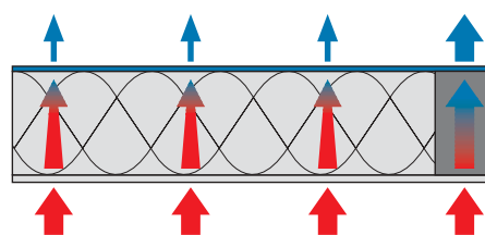
■ Heat loss in roofs without AGEPAN THD.
